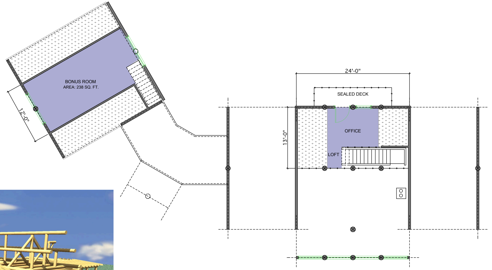
SECOND FLOOR PLAN AREA: 108 SQ. FT.
